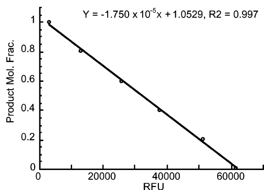
Figure 4. Mole fraction of product 8 versus fluorescence intensity ( \lambda_{\text{excitation}}/\lambda_{\text{emission}} = 360 \text{ nm}/460 \text{ nm} ) for solutions of product 8 , fluorophore 3 , and quencher 7 at a total concentration of 10 -5 M containing 0.0, 0.2, 0.4, 0.6, 0.8, and 1.0 mol fraction of 8 .
